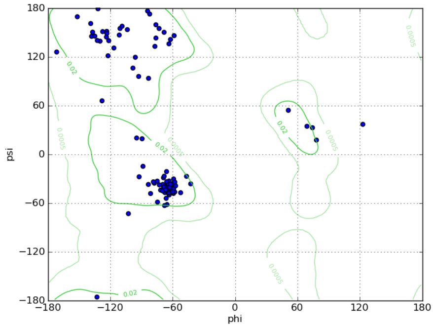
Figure S1. The Ramachandran plot of MsepCSP5
