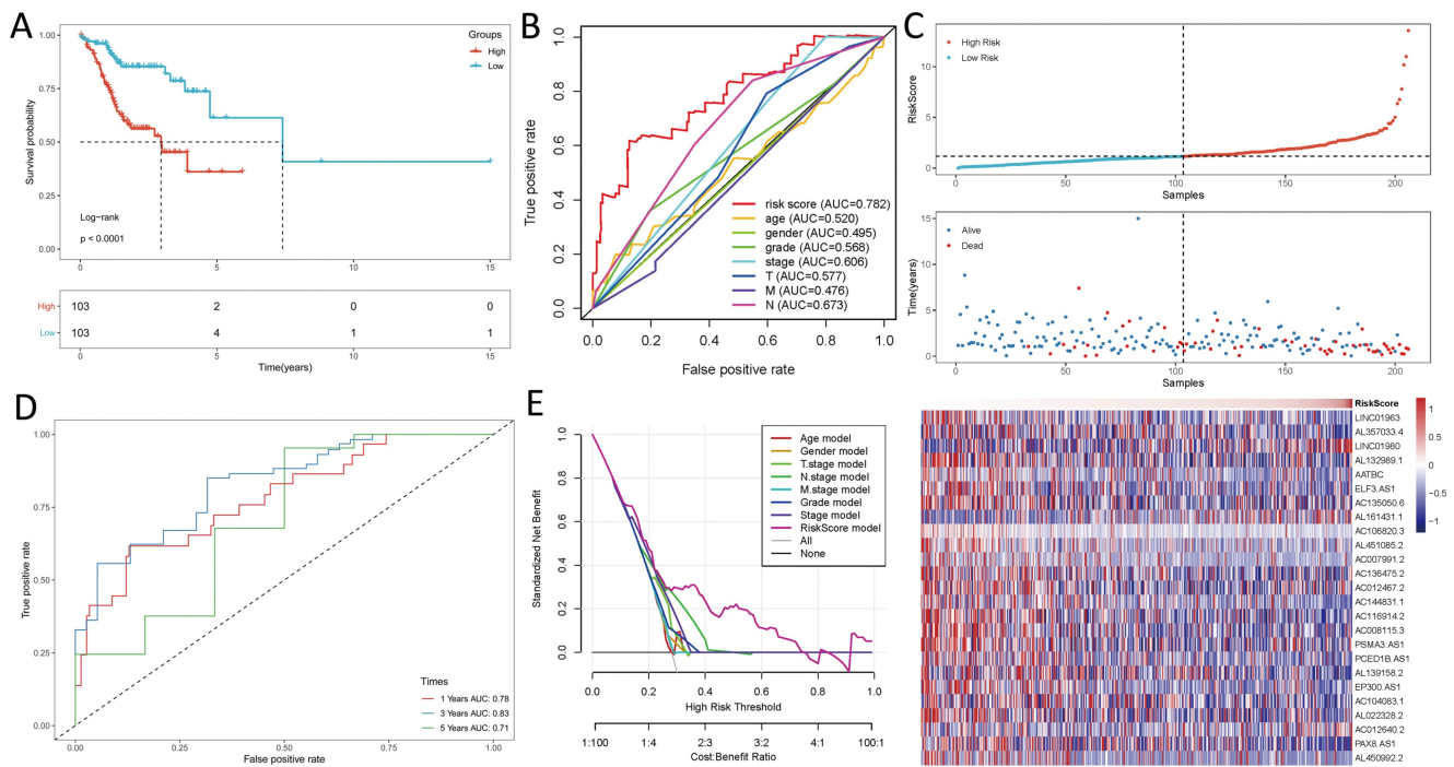
Figure 2. Ferroptosis-related lncRNAs signature based on TCGA. (A) Kaplan-Meier curves result, (B). The AUC values of the risk factors, (C). Risk survival status plot, (D) The AUC of the for the prediction of 1, 3, 5-year survival rate of HNSCC and (E) The DCA of the risk factors.
