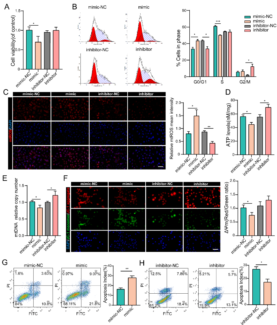
Figure 2. Correct image.
